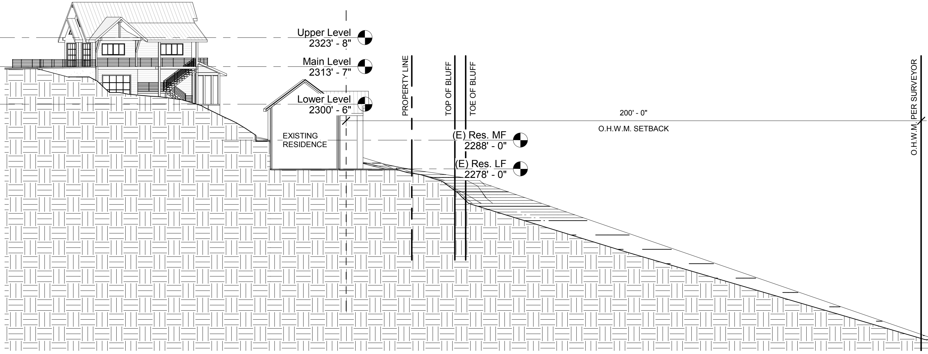
1 Site Section 1" = 20'-0"
